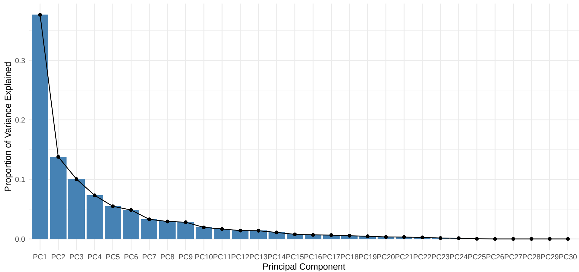
Scree Plot of PCA for FLARE007
